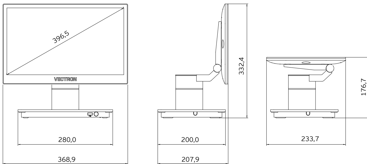
Vectron POS 7 base
